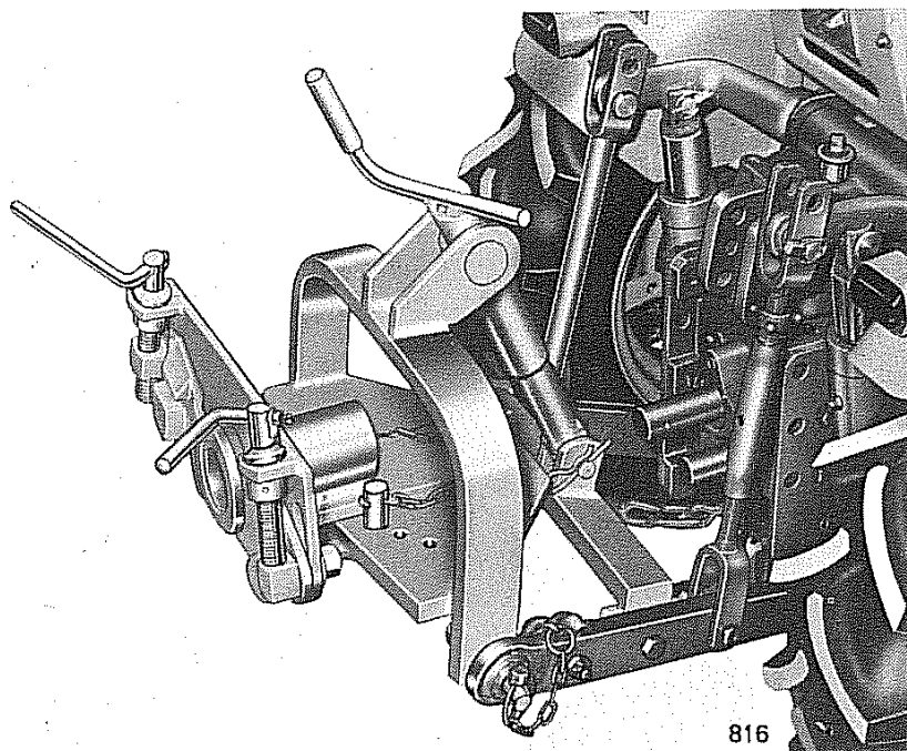
Fig. 91 - Porta aratri universale mod. "2PS20"
